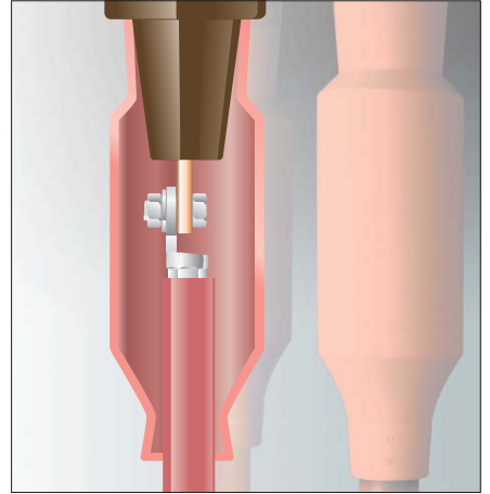
Raychem inline application RCAB up to 24 kV
